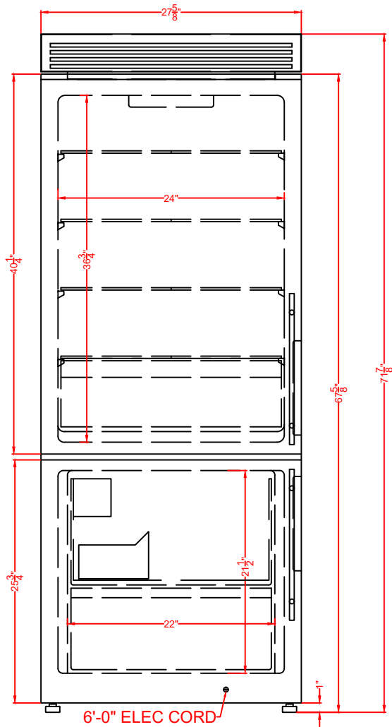
FRONT VIEW
