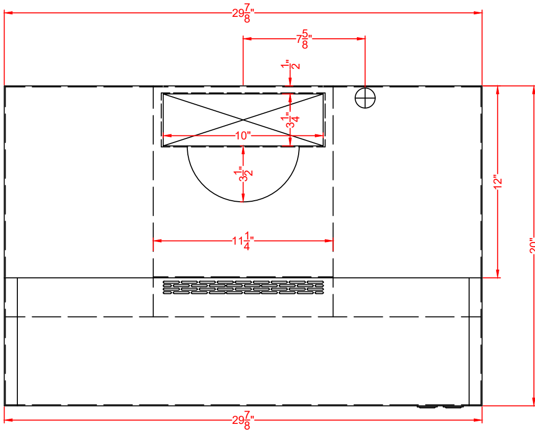
TOP VIEW
