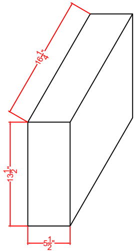
Rack Dimensions (2 Included w/ AULT50PSR12)
