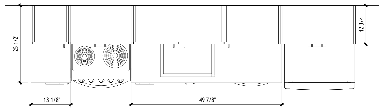
② CABINET PLAN 3/4" = 1'-0"
