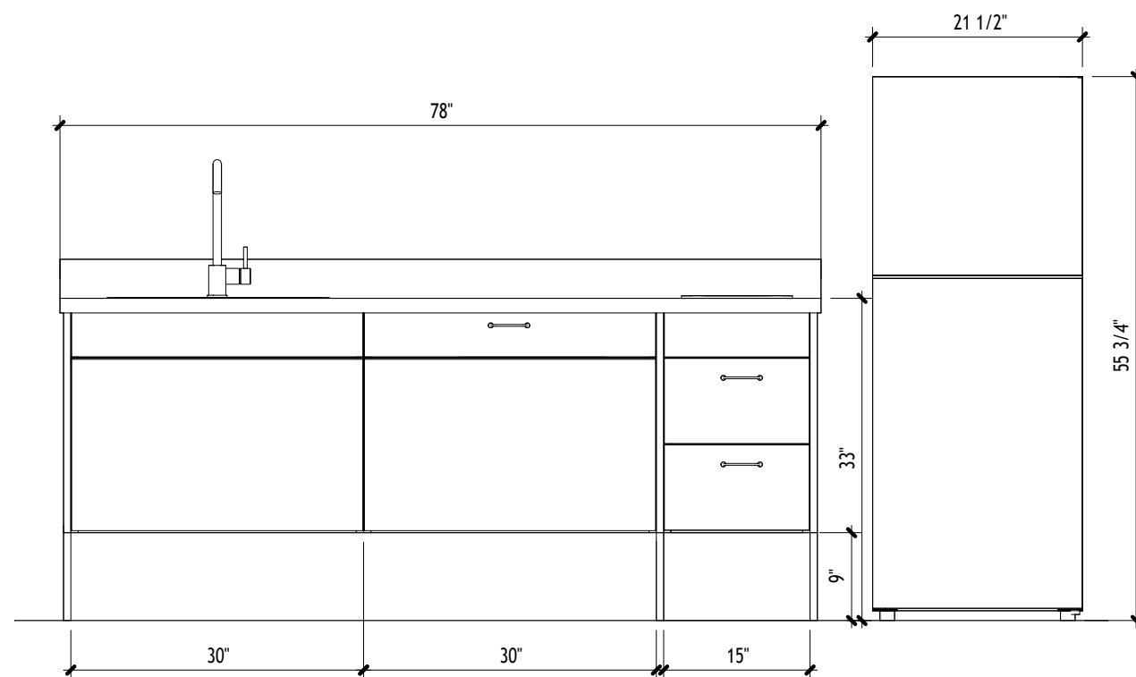
① CABINET ELEVATION 3/4" = 1'-0"
