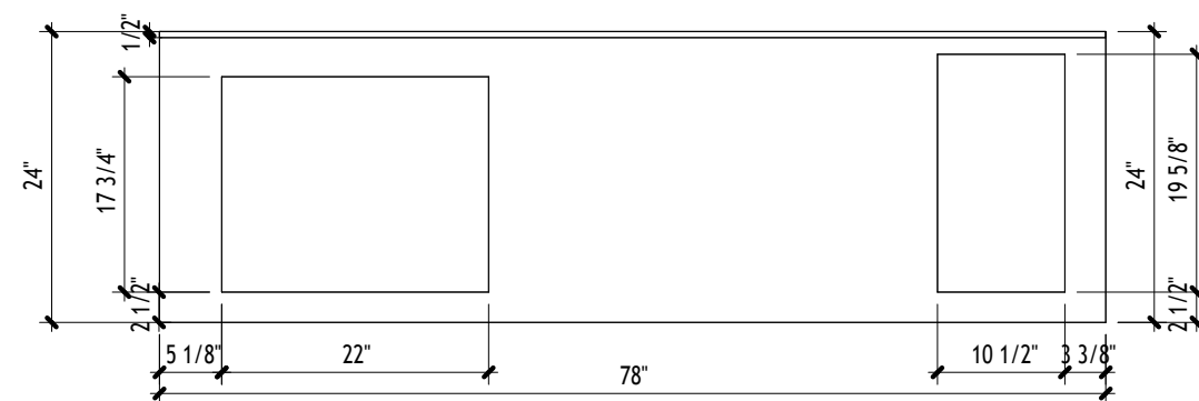
③ COUNTERTOP PLAN 3/4" = 1'-0"
