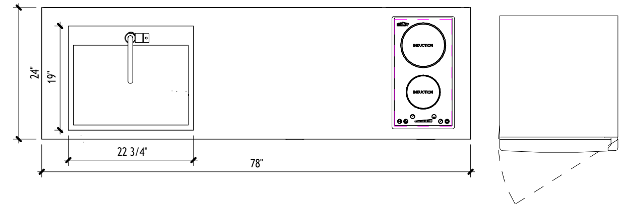
② CABINET PLAN 3/4" = 1'-0"
