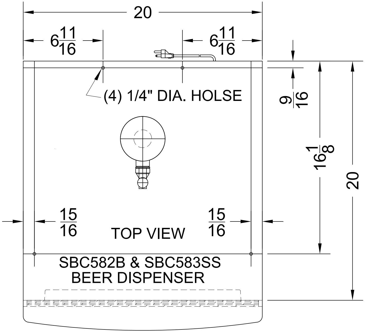
GUARD HOLES LOCATION
